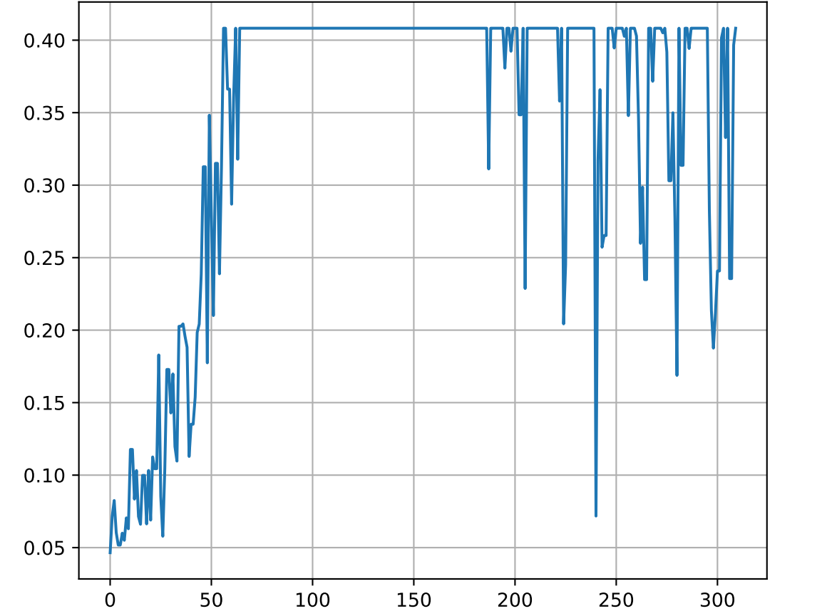
Evaluation Metrics
